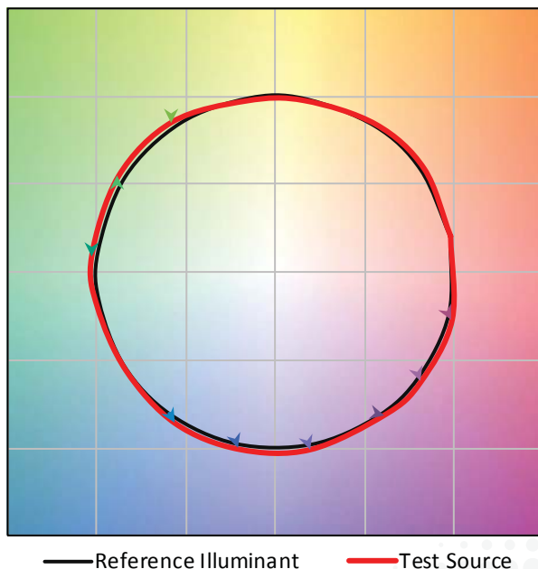
TM 30-15
